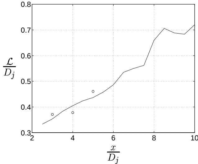
Figure 7.62: Axial development of the integral length scale in the shear layer, i.e. r = 0.5D_j . ' \circ ' denotes experiments (Jordan, 2003).
