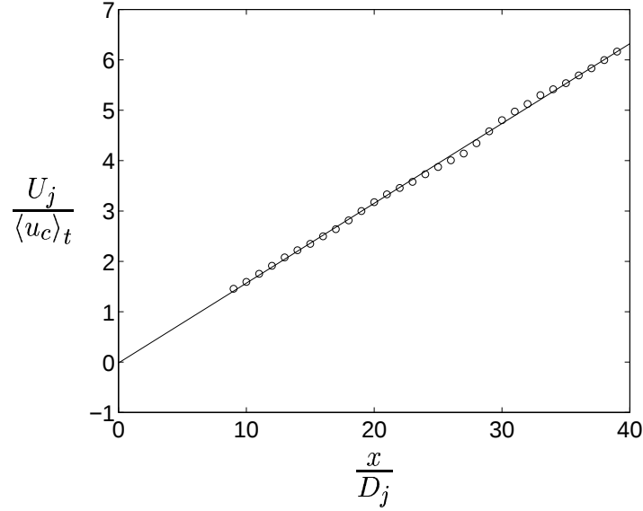
Figure 7.12: Predicted centerline velocity. The solid line corresponds to a curve fit to the LES data. The x -value for which the line intersects the x -axis, x_0 , is used to collapse the radial profiles in figures 7.13–7.17.
