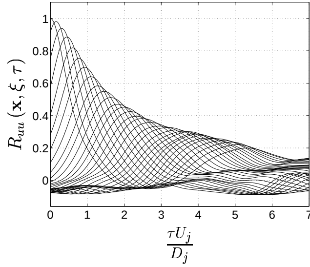
Figure 7.20: Two-point space-time correlation of axial velocity at a location, x , in the shear layer r = 0.5D_j , x = 5.0D_j . See also legend to figure 7.19.
