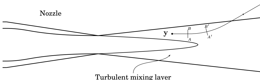
Figure 1.2: Refraction of a sound wave generated at position y in the shear layer and propagating through the jet. A wave front defined by the line AB is propagating downstream at a velocity defined by the speed of sound and the local flow velocity. The flow velocity is higher in A than in B , which results in a tilting of the wave front towards line A'B' .
