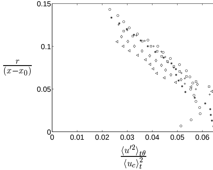
Figure 7.51: Radial profiles of \langle u'u' \rangle_{t\theta} normalized by centerline mean velocity. Radial profiles at six axial locations are represented. The profiles are labeled as follows: ' \circ ' = 29D_j , ' * ' = 31D_j , ' + ' = 33D_j , ' \square ' = 35D_j , ' \diamond ' = 37D_j and finally ' \triangle ' = 39D_j .
