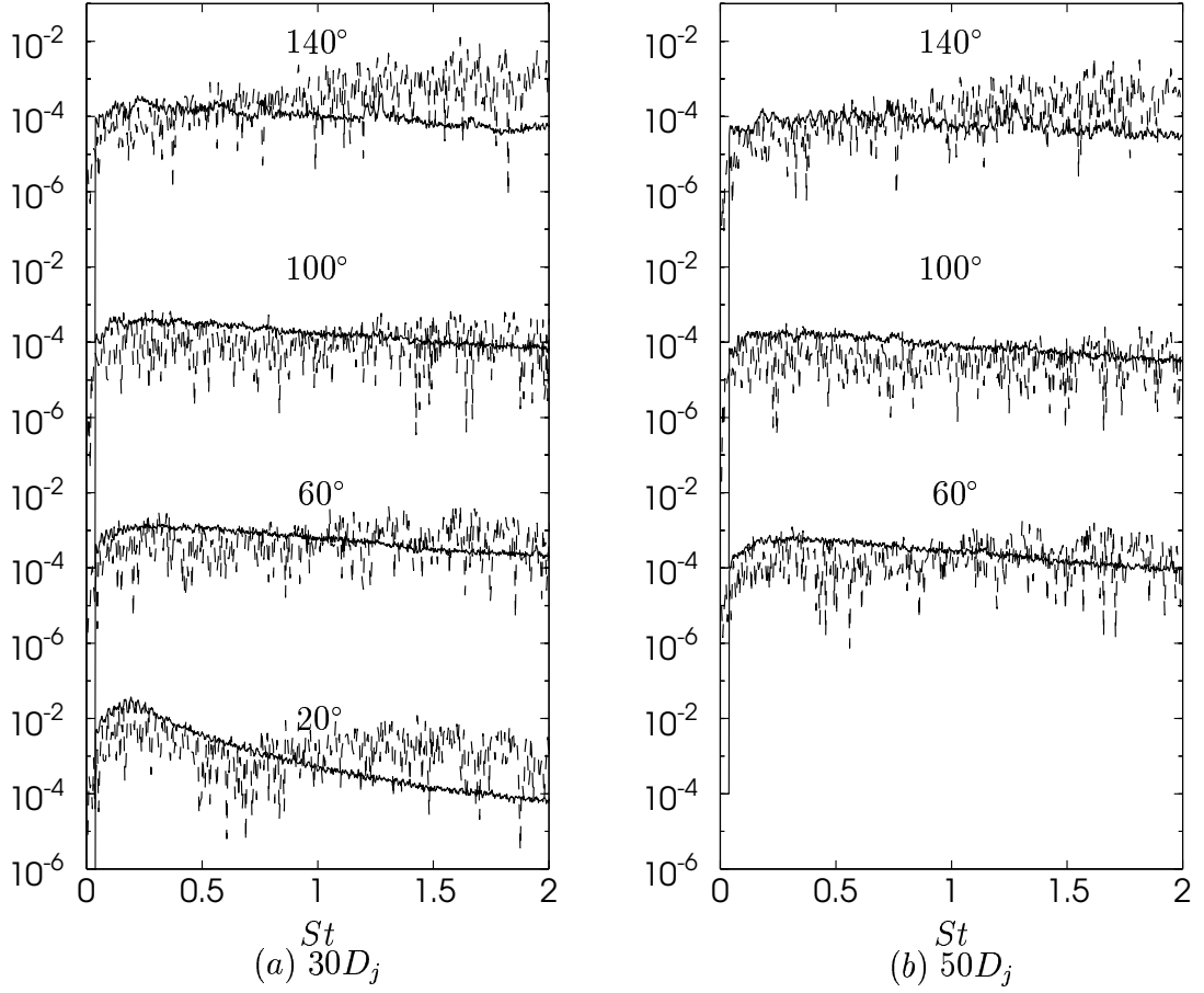
Figure 7.75: Power spectrum of far-field pressure fluctuations versus Strouhal number, St = fD_j/U_j , for Jet I. The dashed line, ' - - ' corresponds to data obtained using Lighthill's acoustic analogy in the temporal derivative formulation and the solid line corresponds to experimental data measured by Jordan et al. (2002b). In figure (a), four observer locations are represented. Starting at a location 20° from the x -axis the angle is increased by an increment of 40° per spectrum. In figure (b) the first spectrum from below is obtained for an observer location 60° from the x -axis, i.e. it should be compared with the second spectrum from below in figure (a). Note that the spectra have been staggered and the scale on the y -axis is therefore repeated.
