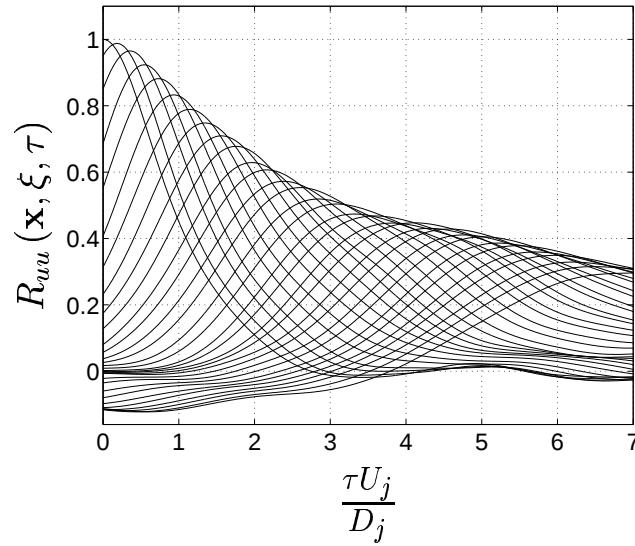
Figure 7.21: Two-point space-time correlation of axial velocity at a location, x , in the shear layer r = 0.5D_j , x = 10.0D_j . See also legend to figure 7.19.
