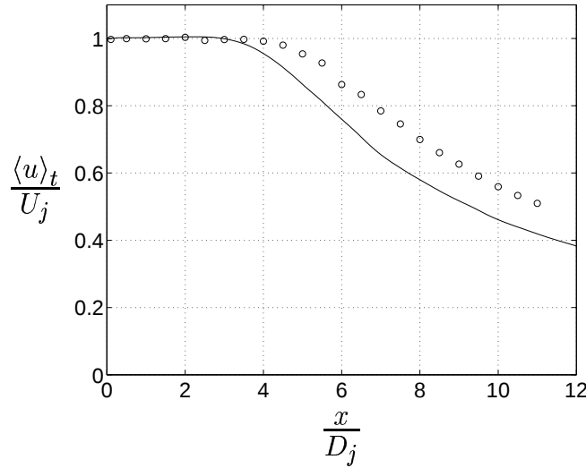
Figure 7.38: Centerline velocity: the solid line, '—', corresponds to LES results and the circles, 'o', to experimental data (Jordan et al. , 2002a).
